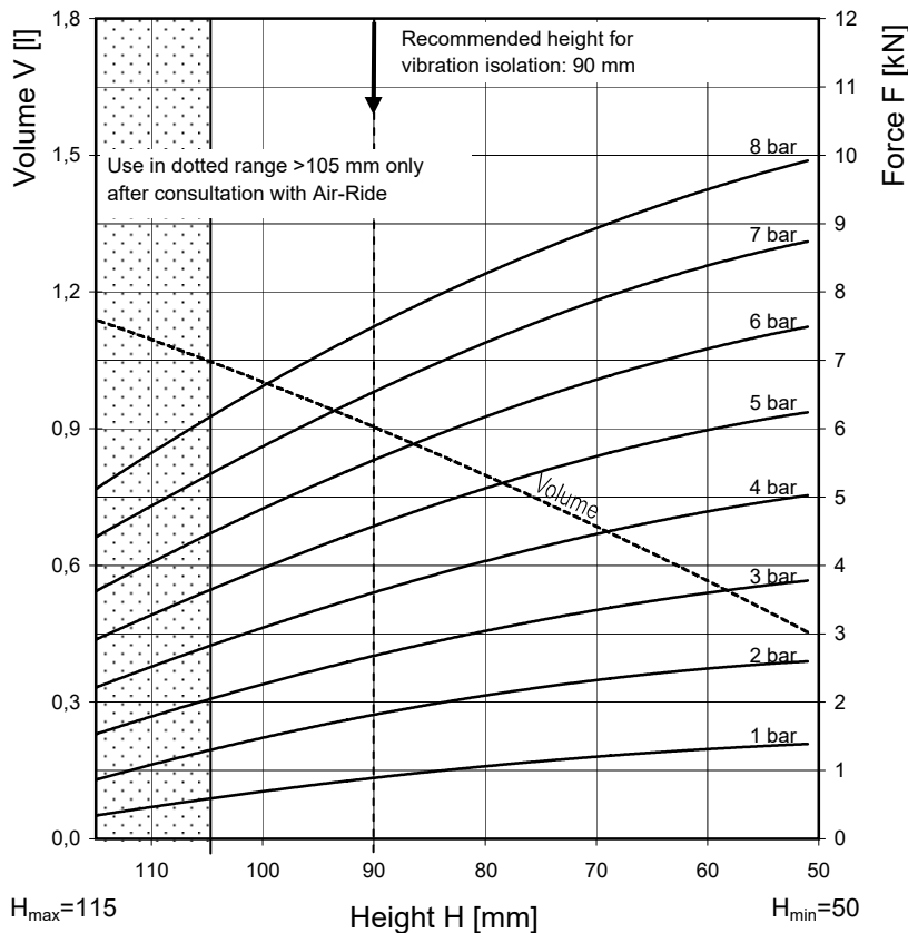
Force-height diagram
