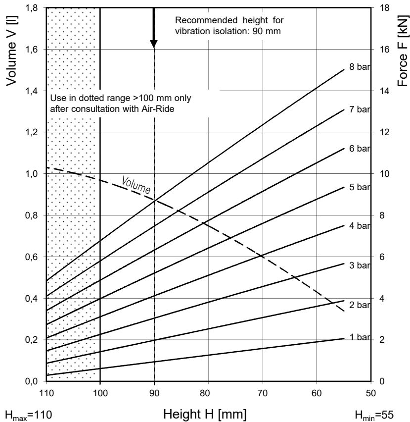
Force-height diagram
