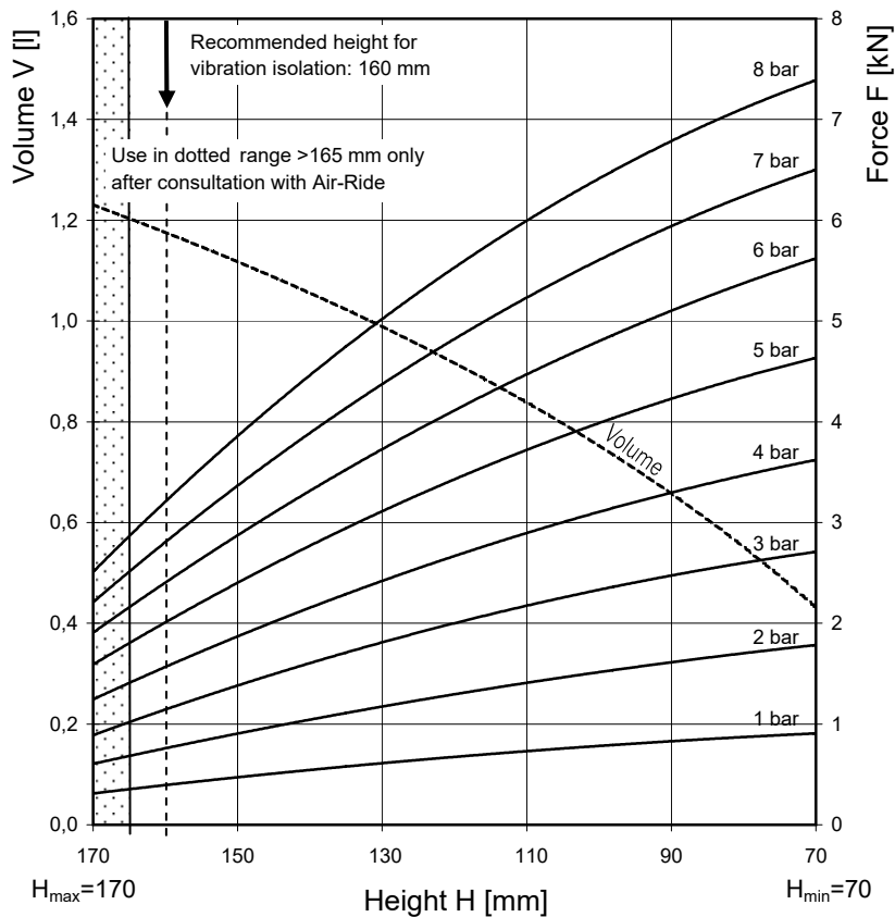
Force-height diagram
