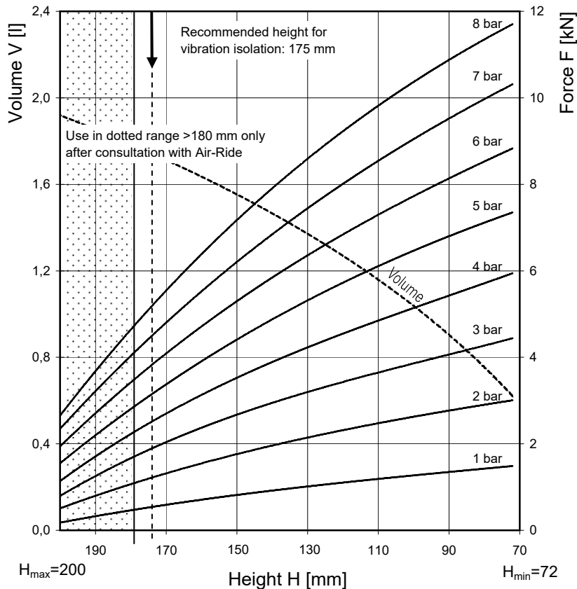
Force-height diagram
