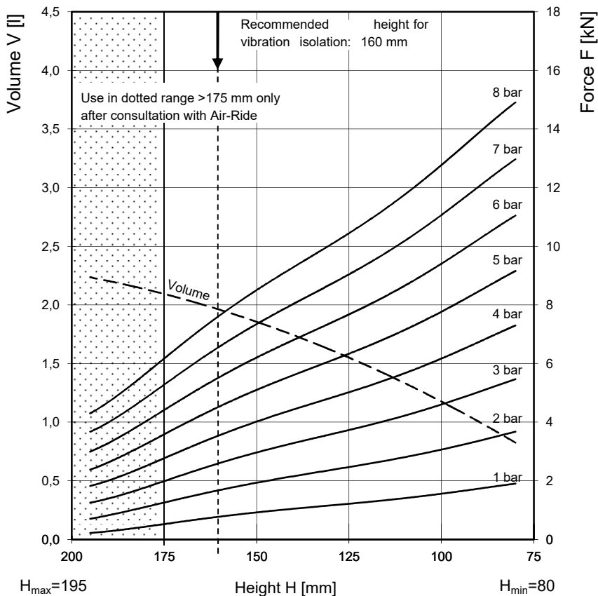
Force-height diagram
