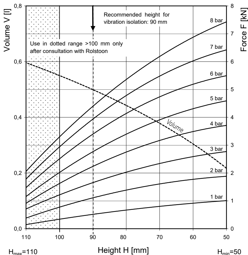
Force-height diagram
